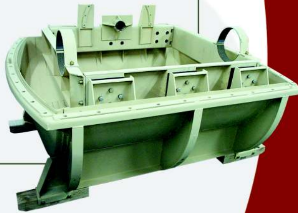
Transmission Shipping Container (upper panel removed) with shock isolation mounting frame
